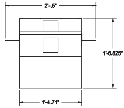
LAYOUT PLAN
