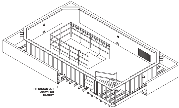
ISOMETRIC PLAN
