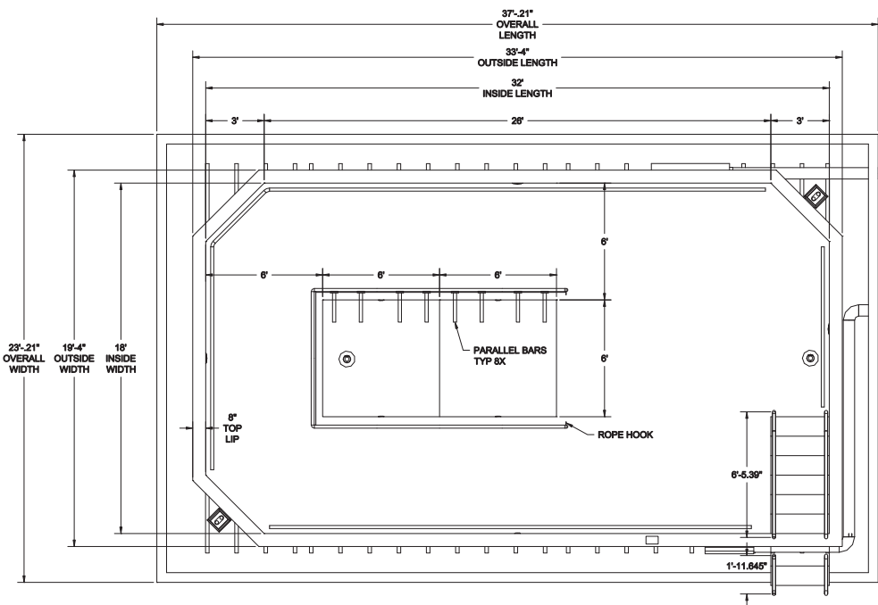
LAYOUT PLAN
