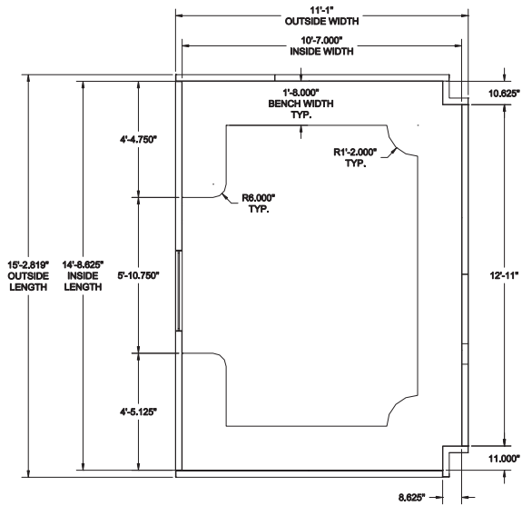
LAYOUT PLAN
