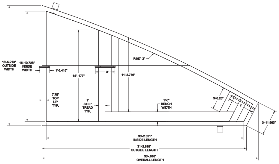
LAYOUT PLAN
