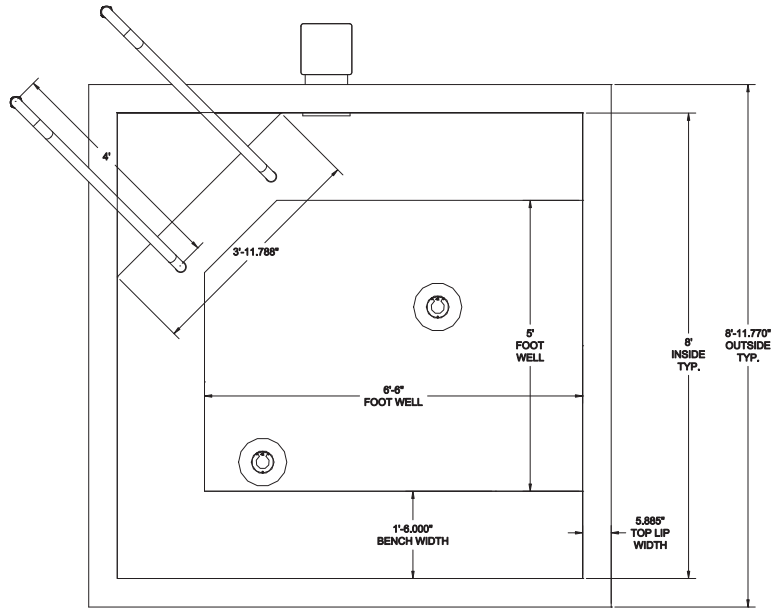
LAYOUT PLAN
