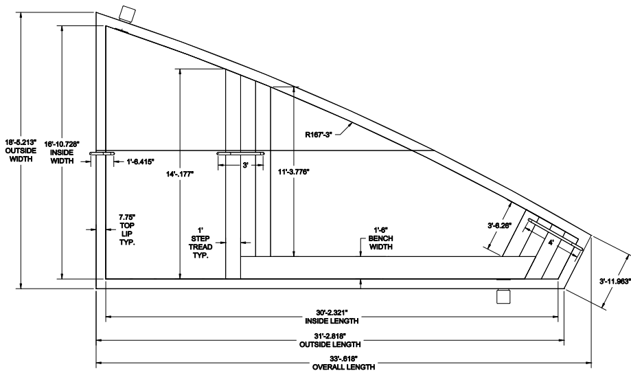
LAYOUT PLAN
