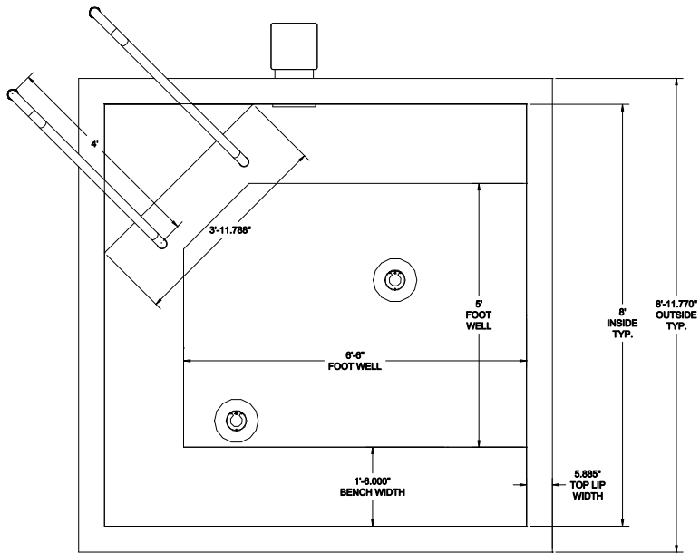
LAYOUT PLAN
