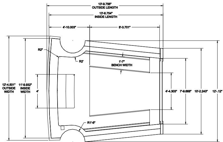
LAYOUT PLAN
